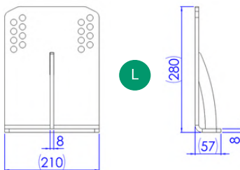
Fixation étroite | Narrow attachment
