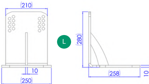
Fixation standard | Main fixing
